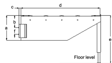
SKV (Pivot mounted – permanent assembly)
