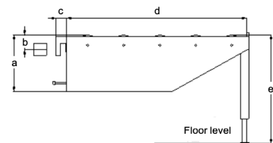
AKV (Hook mounted - detachable)
