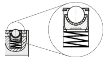
KLF – springloaded ball bar
